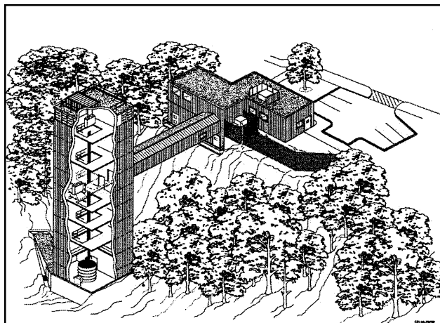
Schematic of the NASA Lewis Research Center 2.2 Second Drop Tower.
