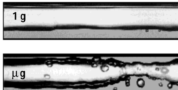
Side views of water and air flowing through a clear pipe. At 1g, the air stays on top. In microgravity, the air can form a core down the center of the pipe.
