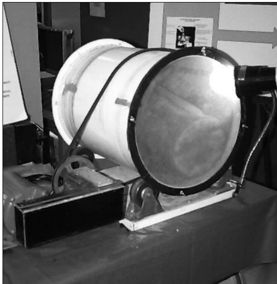
Fabric abrasion tester in use at the NASA Johnson Space Center. The white drum contains an inflated cylinder made from the outer fabric of a spacesuit. The drum also contains lunar sediment simulant. An electric motor with a pulley drives the drum.
